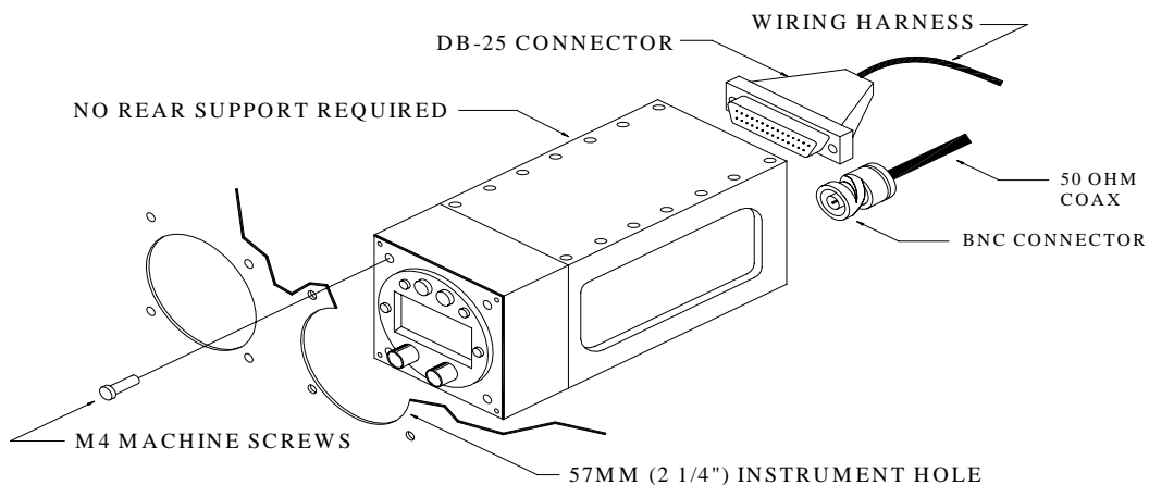
MICROAIR T2000 SFL PANEL INSTALLATION
